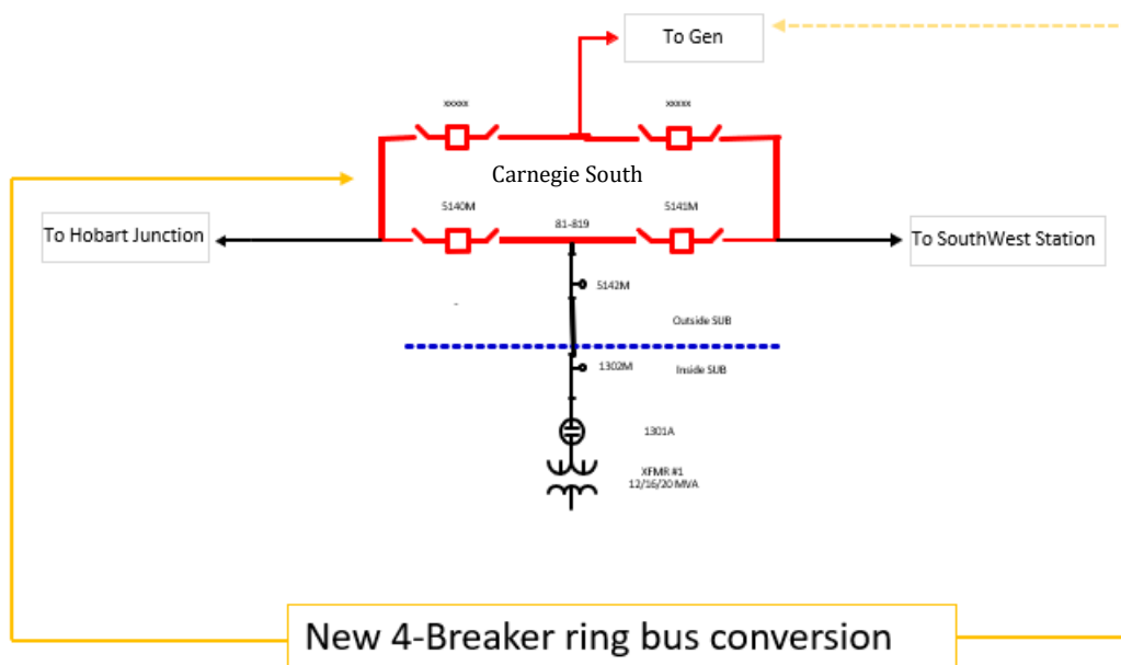
Figure 1: Point of Interconnection (POI INFORMATION) One-Line Diagram
